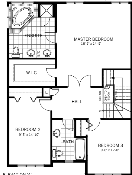
ELEVATION 'A' SECOND FLOOR PLAN - 1,032 sq.ft. (OPTIONAL)
