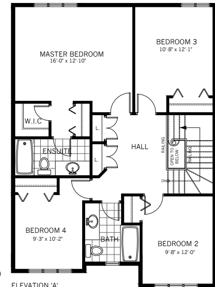
ELEVATION 'A' SECOND FLOOR PLAN - 1,032 sq.ft.
