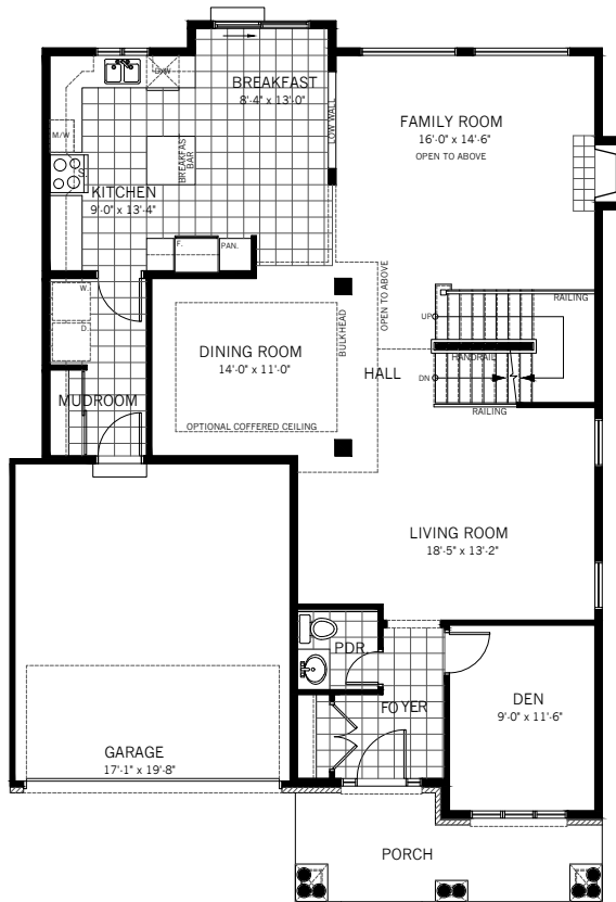
GROUND FLOOR PLAN - 1,322 Sq.Ft. ELEVATION A
