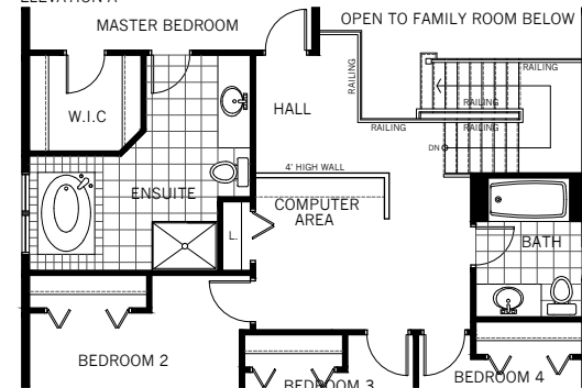
SECOND FLOOR PLAN - OPTIONAL - ELEVATION 'A'
