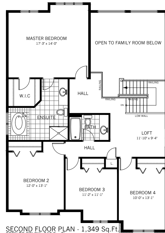
SECOND FLOOR PLAN - 1,349 Sq.Ft. OPEN TO BELOW: 243 Sq. Ft. ELEVATION A
