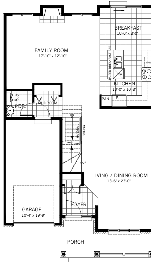
GROUND FLOOR PLAN - 973 sq. ft. ELEVATION 'A'
