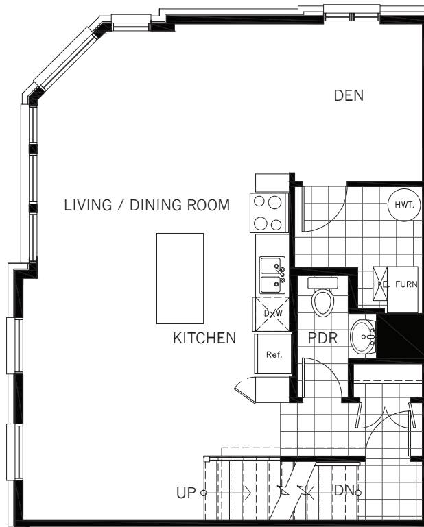
SECOND LEVEL PLAN - 725 sq. ft.
