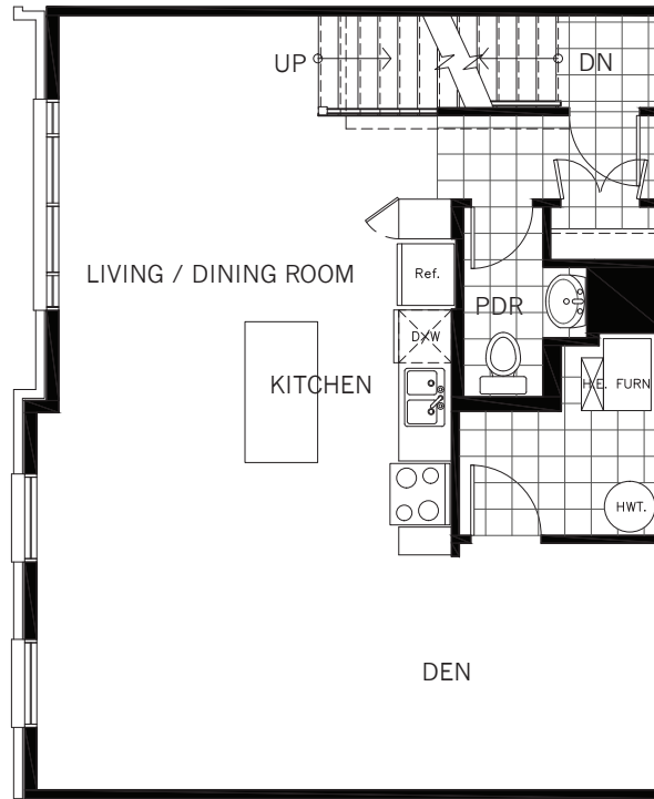
SECOND LEVEL PLAN - 731 Sq Ft
