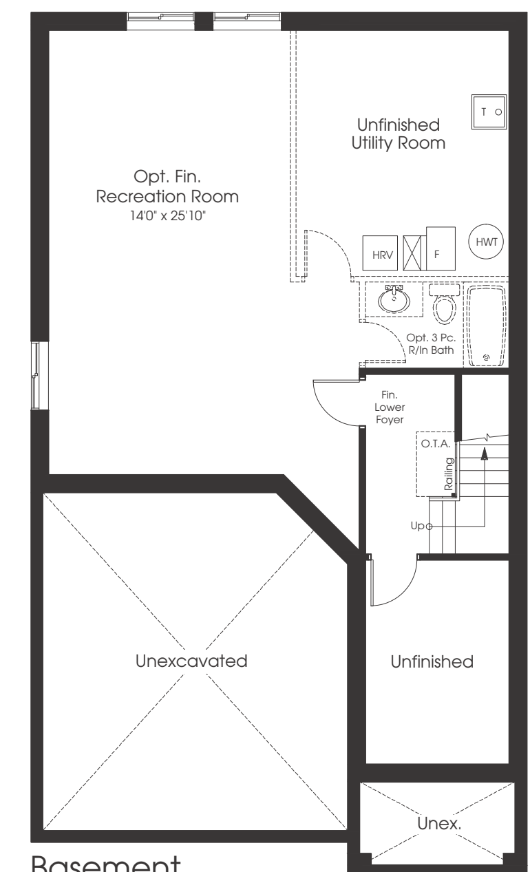
Basement Elev. A
